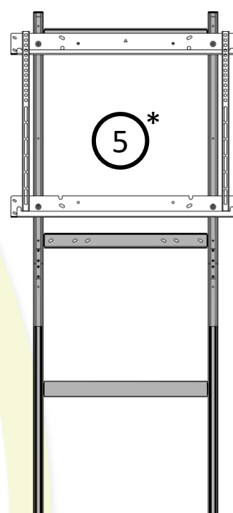
Mounted on Floor support of the BalanceBox®650 (481A13)
